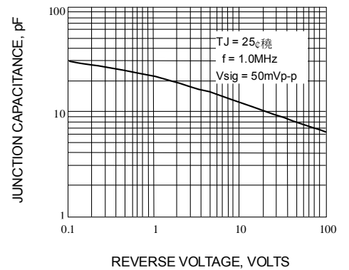
Fig. 6-TYPICAL JUNCTION CAPACITANCE
